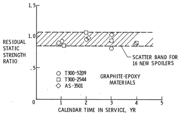
Figure 2.- Residual static strength of graphite-epoxy spoilers.
