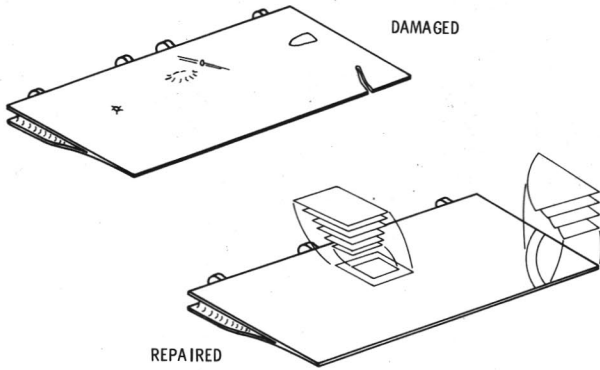
Figure 6.- Graphite-epoxy spoiler repair techniques.
