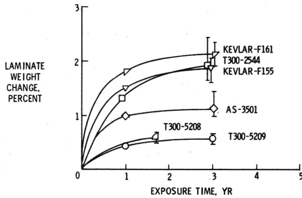
Figure 13.- Moisture pickup after worldwide exposures.
