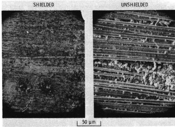
Figure 12.- Graphite-epoxy surface degradation; 3-years outdoor exposure.
