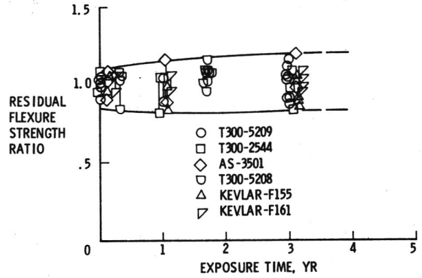
Figure 15.- Residual flexure strength after worldwide exposure.
