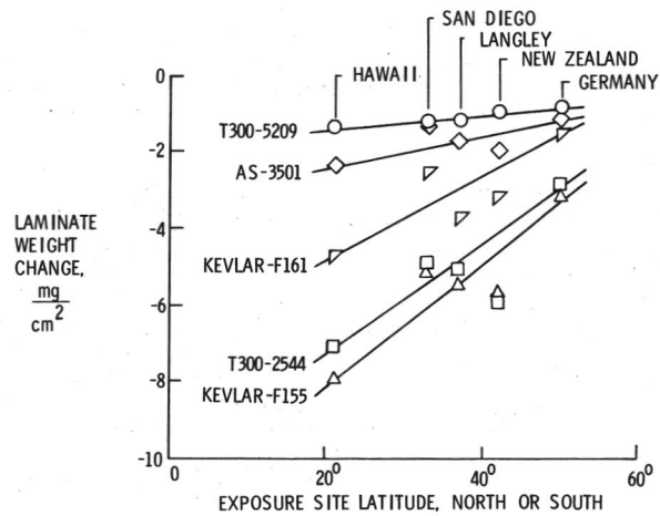
Figure 11.- Weight loss from three-years outdoor ultraviolet exposure.
