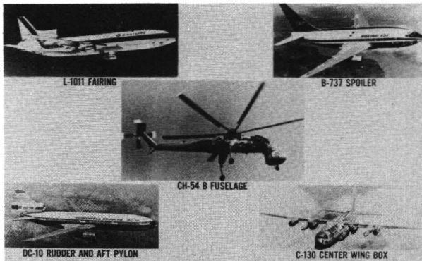
Figure 1.- Flight service evaluation of composite structural components.
