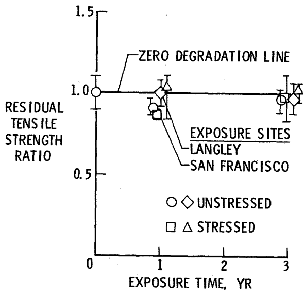
Figure 17.- Residual tensile strength after sustained stress outdoor exposures; T300-5208, (0°, +45°, 90°) laminate stressed at 40 percent ultimate.
