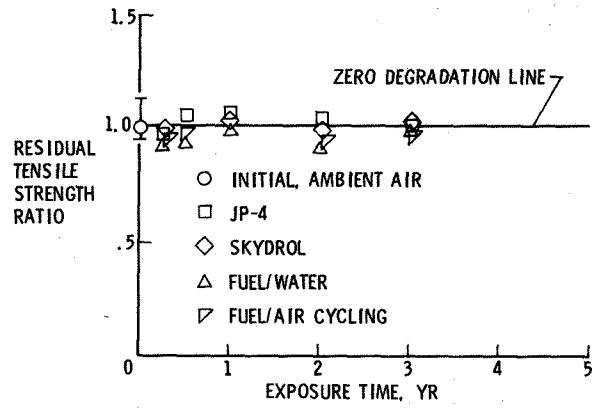
Figure 18.- Effect of fuels and fluids on strength; T300-5209, +45° tensile specimens.
