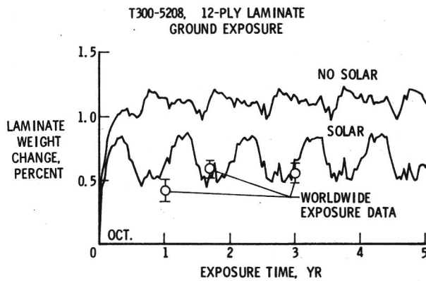
Figure 14.- Comparison of predicted and measured moisture contents; T300-5208, 12-ply laminate; ground exposure.
